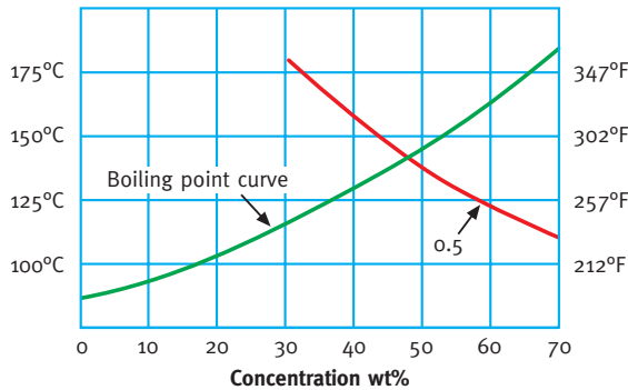
Isocorrosion Curve for FERRALIUM 255-SD50 in Sodium Hydroxide shown at a Corrosion Rate of 0.5mm/y
