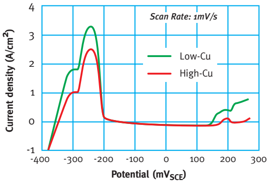
Electrochemical Polarisation Curves in 1M HCl at 65°C of superduplexes of similar composition containing 0.6% Cu (low-Cu) and 1.6% Cu (high Cu)
