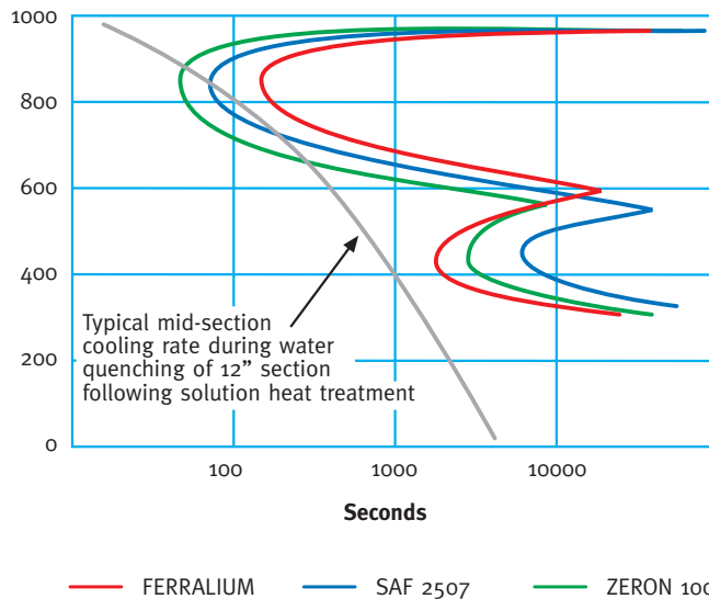
Transformation Time/Temperature for the three main superduplex stainless steels
