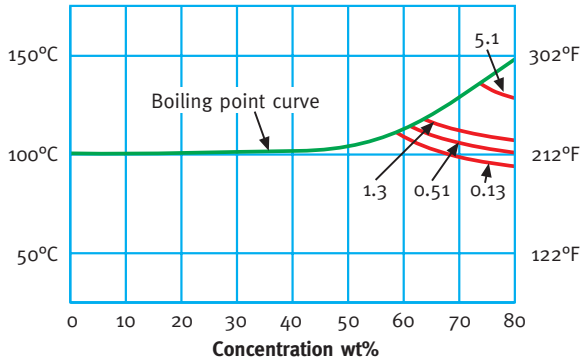
Isocorrosion Curves for FERRALIUM 255-SD50 in Phosphoric Acid shown at Corrosion Rates of 0.13mm/y, 0.51 mm/y, 1.3 mm/y and 5.1mm/y.
