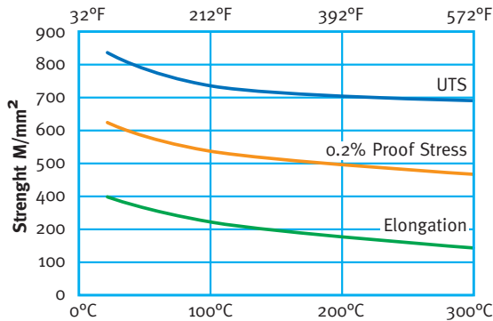
Graph showing the typical mechanical properties of FERRALIUM 255-SD50 at elevated temperatures
