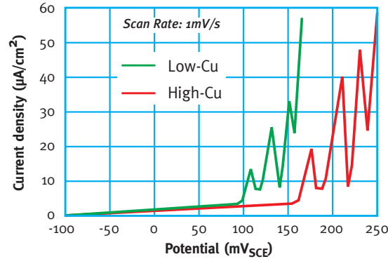
Electrochemical Polarisation Curves in 3.5% NaCl at 65°C of superduplexes of similar composition containing levels of copper at 0.6% (low copper) and 1.6% (high copper)
