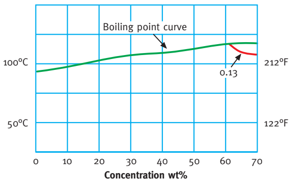
Isocorrosion Curve for FERRALIUM 255-SD50 in Nitric Acid shown at a Corrosion Rate of 0.13mm/y.
